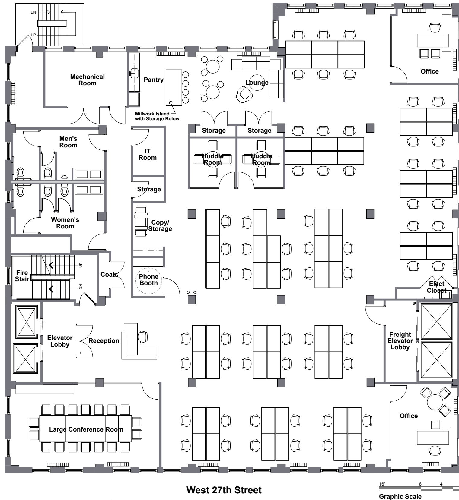
3rd Floor Fit Plan - Option A
